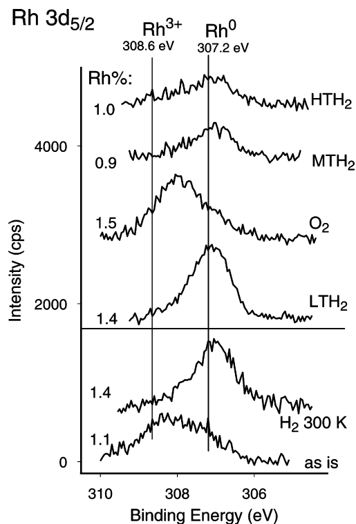
Fig. 4. Rh 3d XP spectra for Rh–Pt catalyst after pretreatments.
