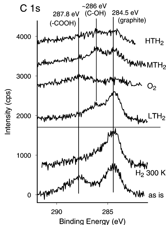
Fig. 6. C 1s XP spectra for bimetallic sample in the “as is” state and after pre-treatments.
