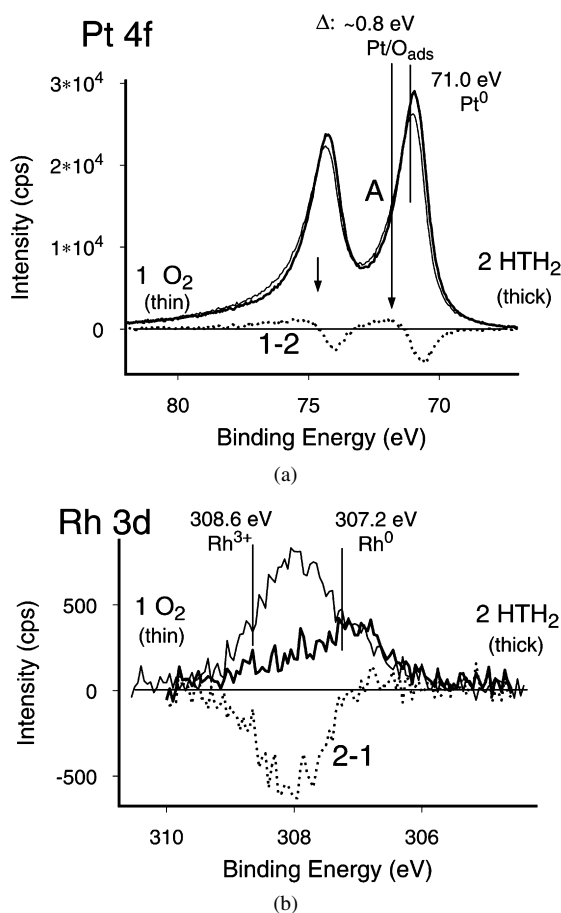
Fig. 5. XP spectra of the Pt and Rh components after O 2 treatment at 573 K and H 2 treatment at 673 K, together with the difference spectra.
