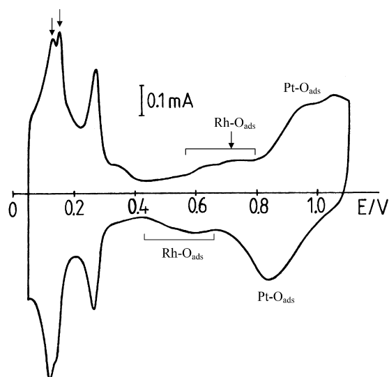
Fig. 1. Cyclic voltammogram of the Rh–Pt catalyst after its preparation. The double peak at \sim 150 mV, the appearance of the adsorption of oxygenates (OH and/or O) at \sim 0.6 eV and the peaks on the cathodic polarization indicate the presence of Rh.
