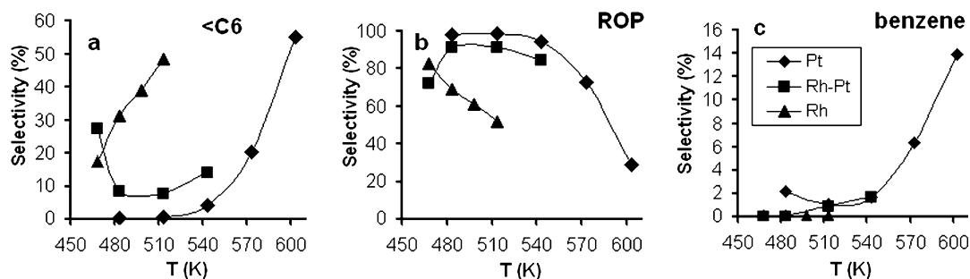
Fig. 7. Selectivity of fragments (a), ring opening products (b), and benzene (c) in MCP transformation on Pt , Rh-Pt , and Rh sample at p(\text{MCP}):p(\text{H}_2) = 1.3:16 kPa, t = 5 min.
