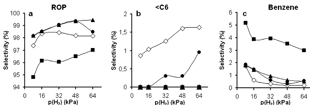
Fig. 9. (a) Selectivity of ring opening products; (b) fragments; (c) benzene on Rh–Pt after the four pretreatments as a function of hydrogen pressure at 513 K, t = 5 min.
