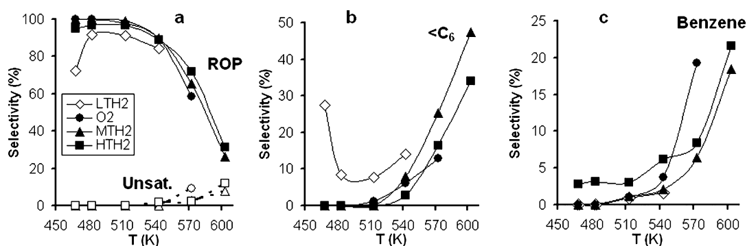
Fig. 8. (a) Selectivity of ring opening (curves in the upper region) and unsaturated products (curves close to the abscissa); (b) fragments; (c) benzene on Rh–Pt after the four pretreatments as a function of temperature at p(\text{MCP}):p(\text{H}_2) = 1.3:16 kPa, t = 5 min.
